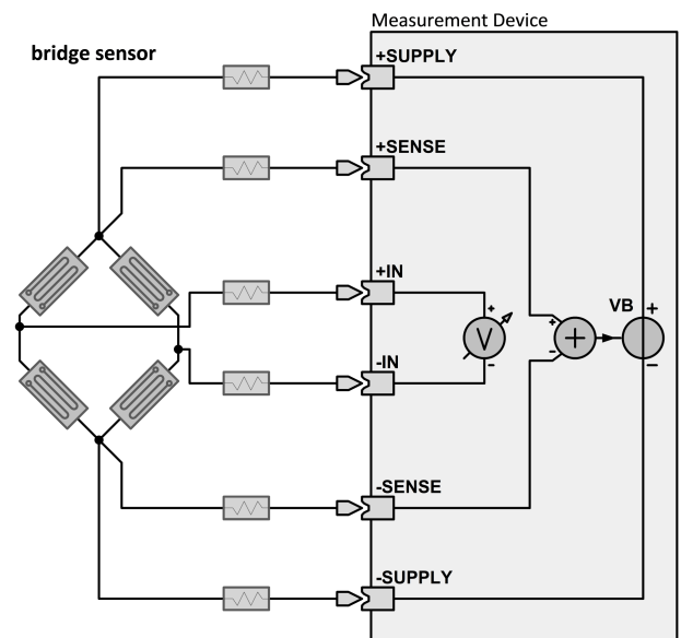
Fig. 34: 6-wire configuration (B-4)
