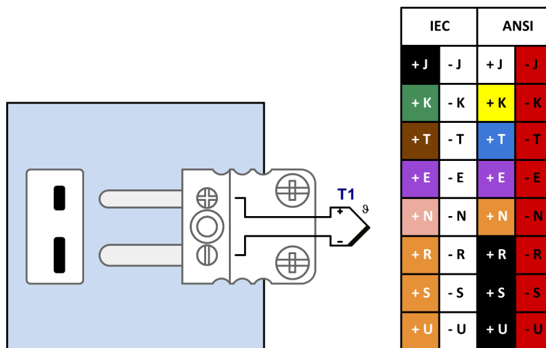
Thermocouple measurement
