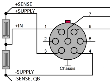
Fig. 29: Connection schematic B-4 half bridge
