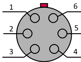
Fig. 43: Remote socket (view on top of the socket)
