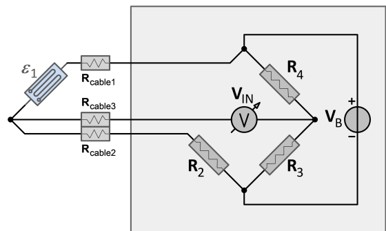
Fig. 26: Quarter bridge in three wire configuration
