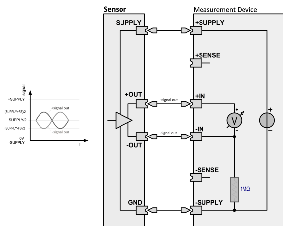
b) sensor with differential output
