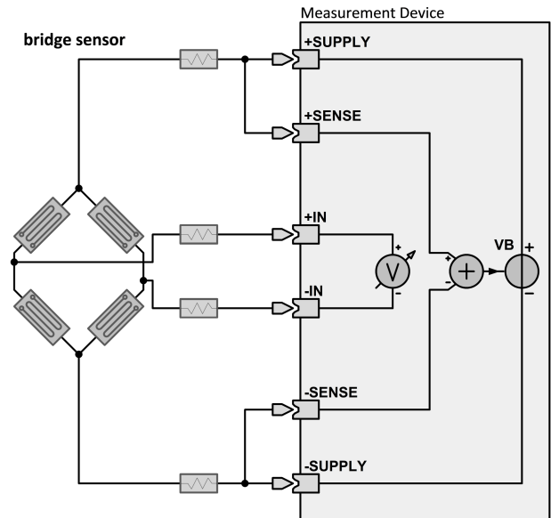
Fig. 33: 4-wire configuration (B-4)
