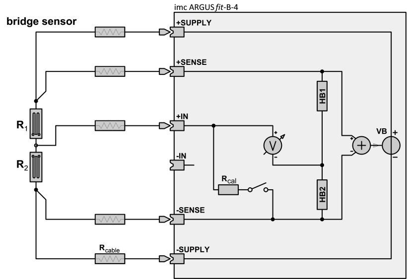
Fig. 30: Block schematic B-4 half bridge
