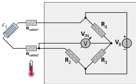
Fig. 25: Quarter bridge in two wire configuration
