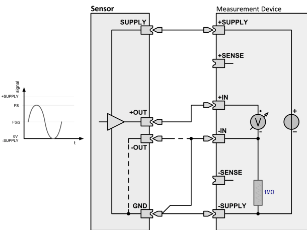
a) sensor with single-end output
