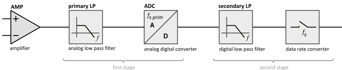
Fig. 15: signal processing chain of the ARGUS series
