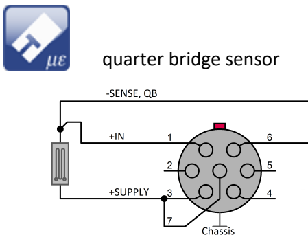
Fig. 27: Connection schematic B-4 quarter bridge
