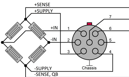
Fig. 31: Connection schematic B-4 full bridge
