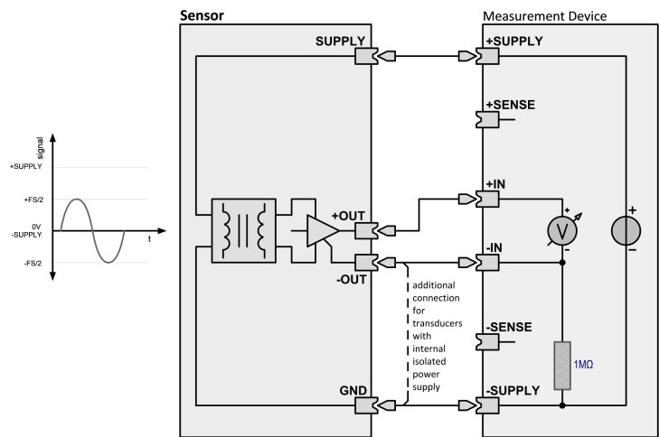
c) sensor with isolated output
