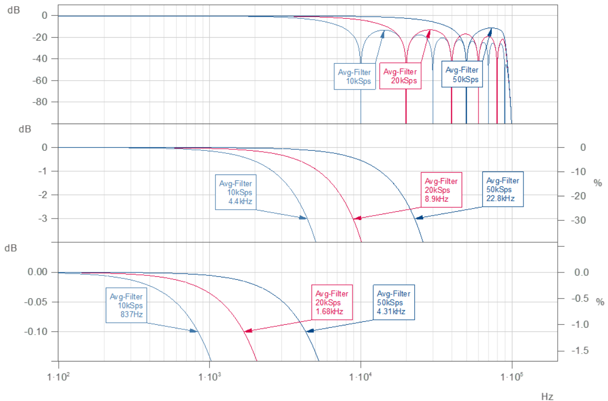
Fig. 21: "Filter type: Average filter" for different sampling rates ( f_{s\_prim} = 200 kSps)
