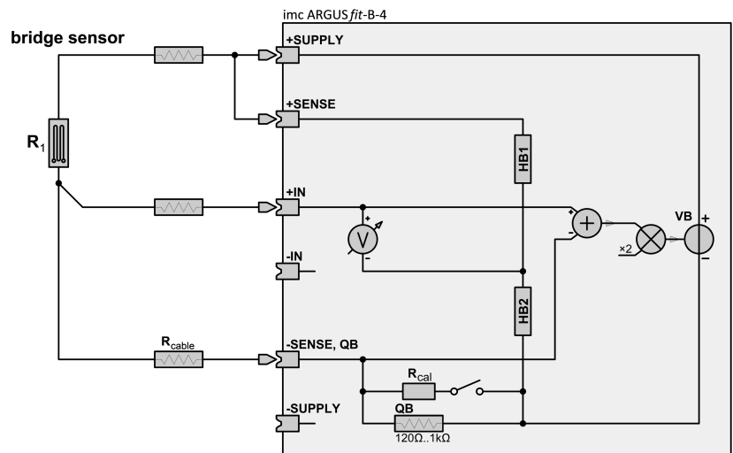
Fig. 28: Block schematic B-4 quarter bridge
