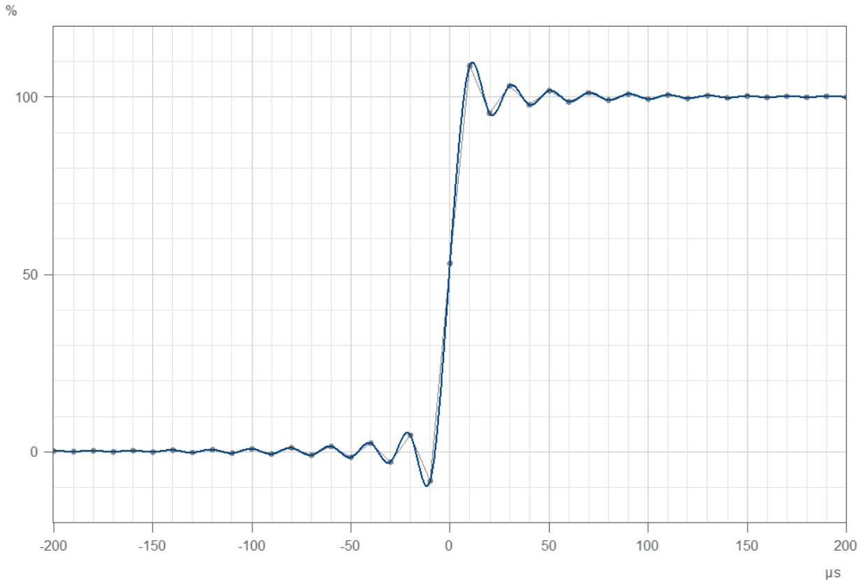
Fig. 24: Step response with "Filter type: without" for ARGFT/ICPU-6 at 500 kSps
