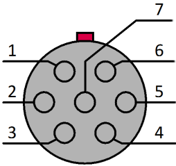
Fig. 44: GPS socket (base unit) (view on top of the socket)
