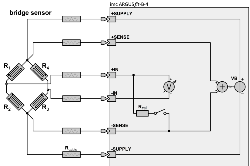
Fig. 32: Block schematic B-4 full bridge
