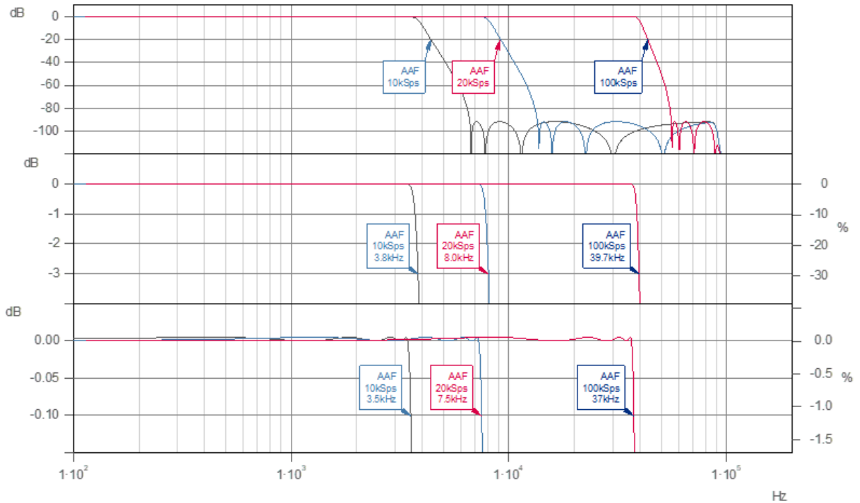
Fig. 20: "Filter type: AAF" (Cauer) for different cut-off frequencies ( f_s prim = 200 kSps)
