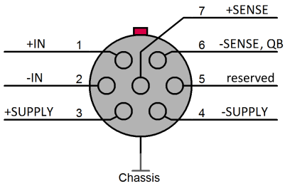
Fig. 46: B-4 socket (pinning) (View on top of the socket)
